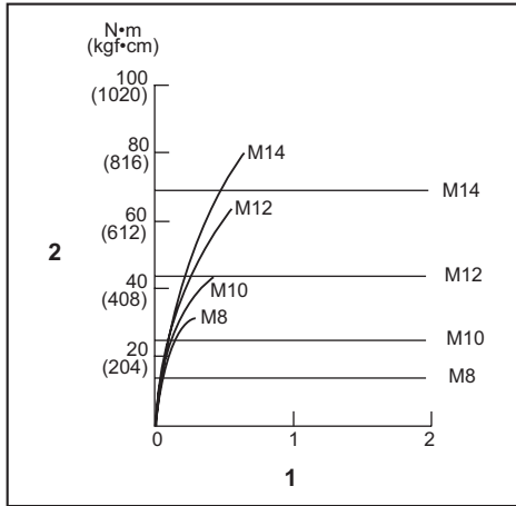
1. Fastening time (seconds) 2. Fastening torque
